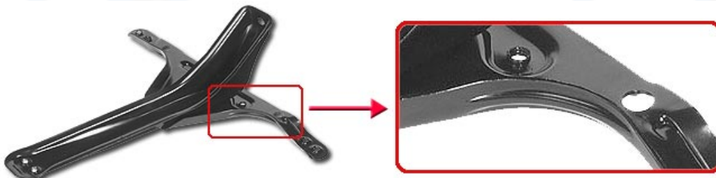
Stiffening ribs
